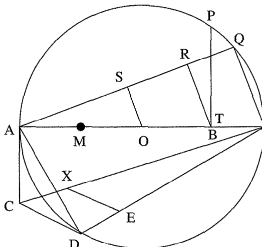
Figure 7.6: Srinivasa Ramanujan's approximate squaring of the circle.
