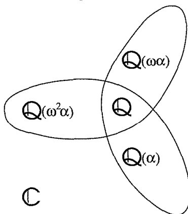
Figure 11.1: \mathbb{Q} -monomorphisms of \mathbb{Q}(\sqrt[3]{2}) : \mathbb{Q} .
