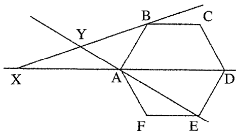
Figure 7.7: Duplicating the cube using a marked ruler.
