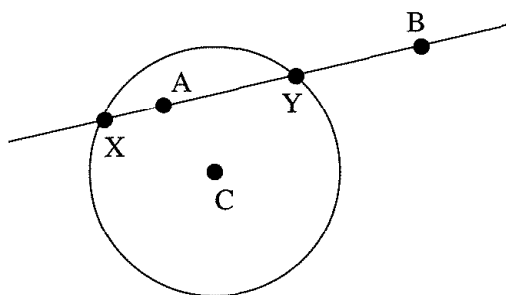
Figure 7.3: Line meets circle.
