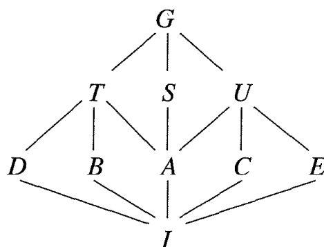
Figure 13.2: Lattice of subgroups.
