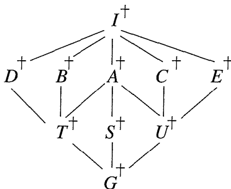
Figure 13.3: Lattice of subfields.
