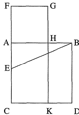
Figure 19.10: Cutting a line in extreme and mean ratio.
