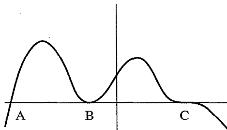
Figure 3.1: Multiple zeros of a (real) polynomial. The multiplicity is 1 at (A), 2 at (B), and 3 at (C).
