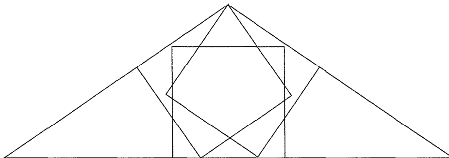
Figure 1.1: Calabi's triangle.
