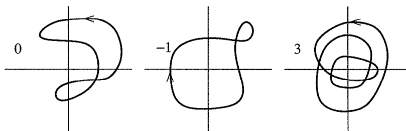
Figure 2.2: Winding numbers.
