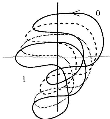
Figure 2.3: How the winding number can change when a deformation of the loop passes through the origin.
