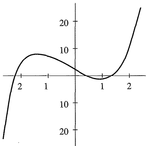
Figure 15.2: A quintic with three real zeros.
