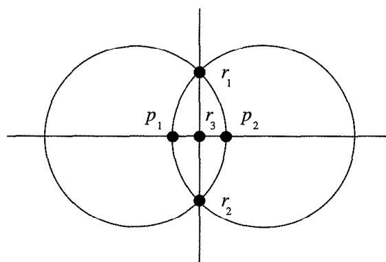
Figure 7.2: Bisecting a line segment with ruler and compasses.
