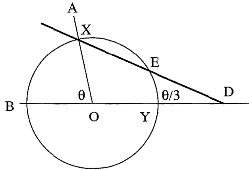
Figure 7.1: Trisecting an angle with a marked ruler.
