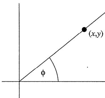
Figure 2.1: Definition of the argument.
