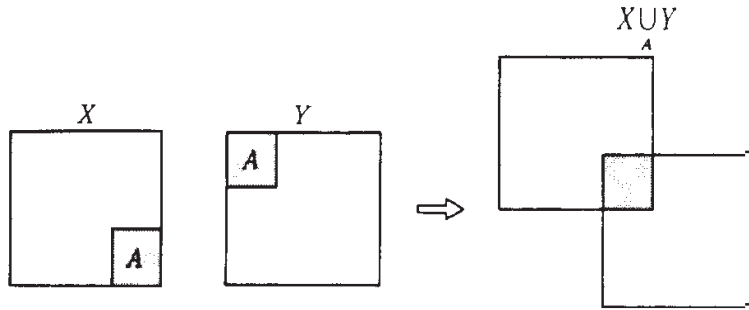
FIGURE 2.2. Topological sum
