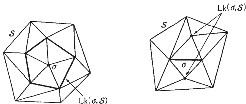
FIGURE 1. Link complex
