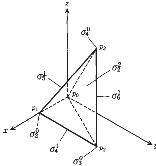
FIGURE 5.1. Simplicial complex
