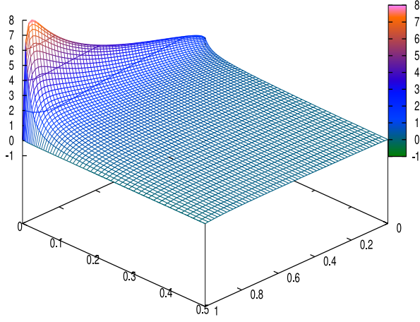
(a) Set 3: f_1(x, y)
