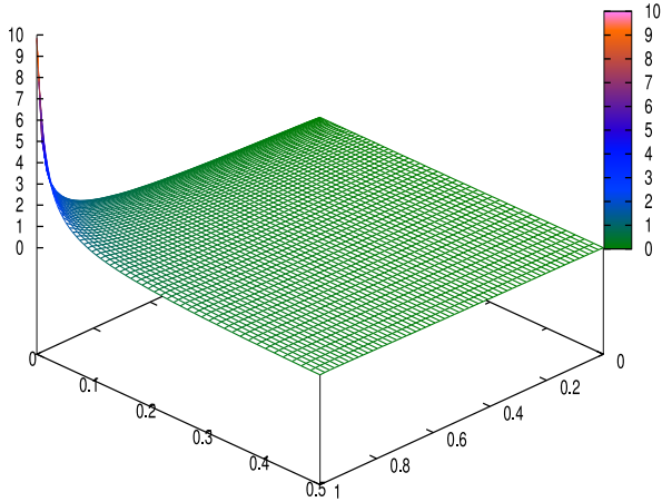
(c) Set 4: f_1(x, y)
