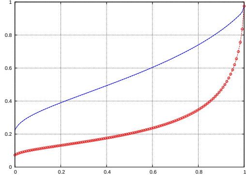
(b) Set 3: f_2(x) (solid) and f_3(x) (circles)
