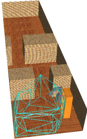
(a) New obstacle location and region C_{id18,2} .
