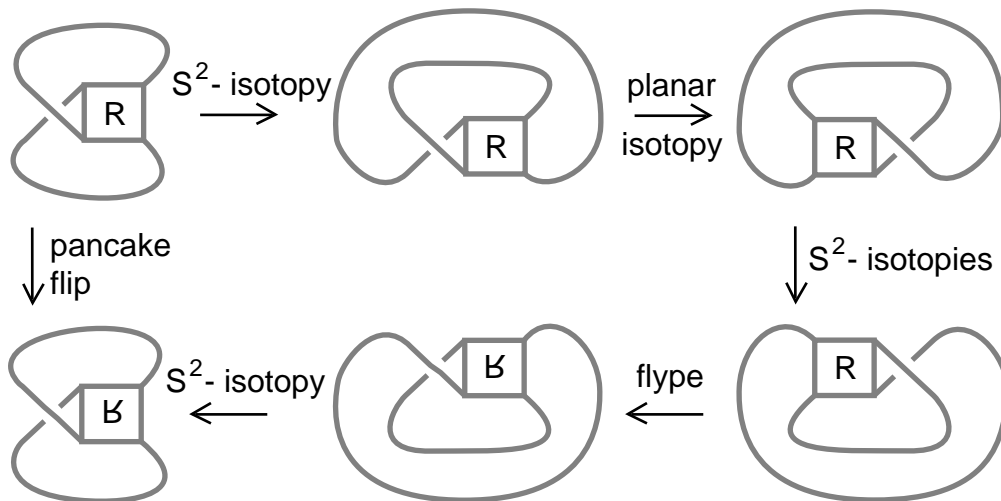
Figure 17 - Pancake flip
