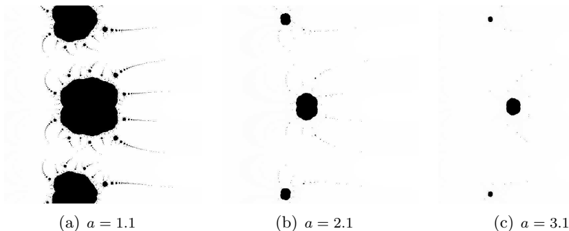
Fig. 1. The Julia set for f_a (and a an escaping parameter) is white, and the Fatou set is black.
